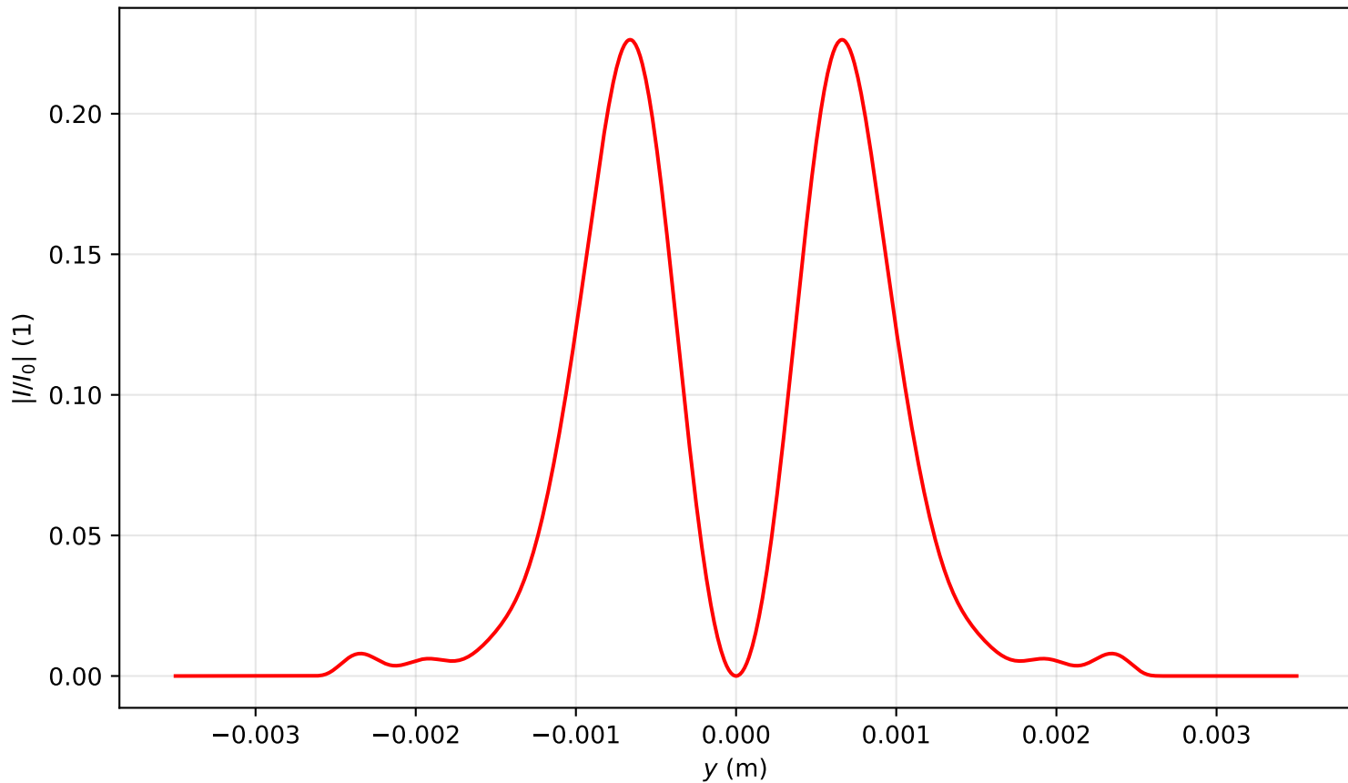
Intensity profile I(x=0, y, z=2.627)/I_0 , P_{in}=4.0P_{cr} , artificial time
